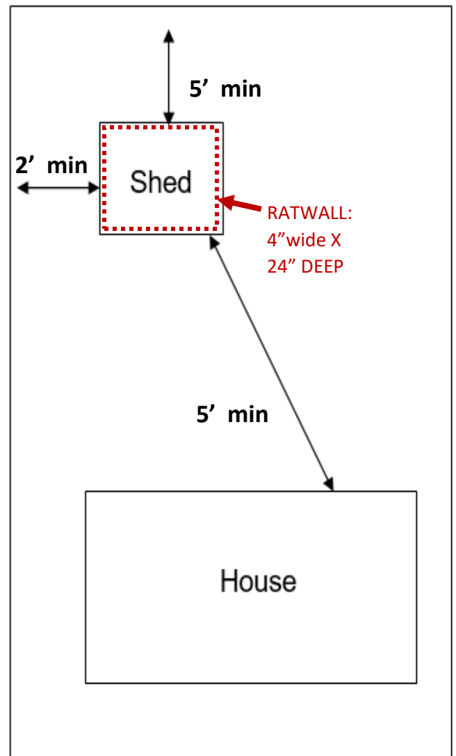
Sample Plot Plan
